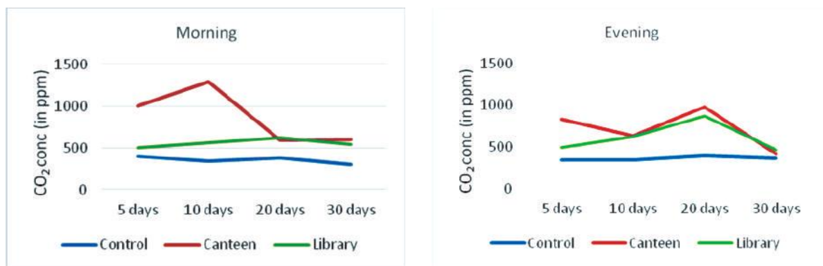
Fig. 20 & 21 Real time measurement of CO 2 concentration (in ppm) at different site upon with keeping 3 plants of areca palm/ site
