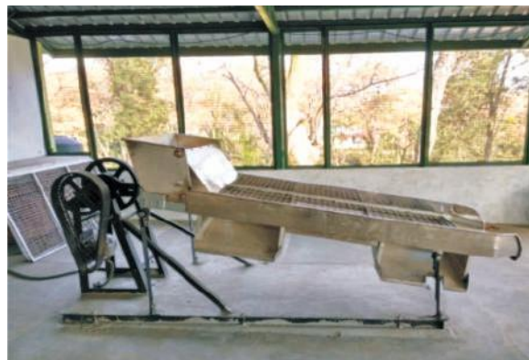
Fig. 36 Tea leaf sorter
