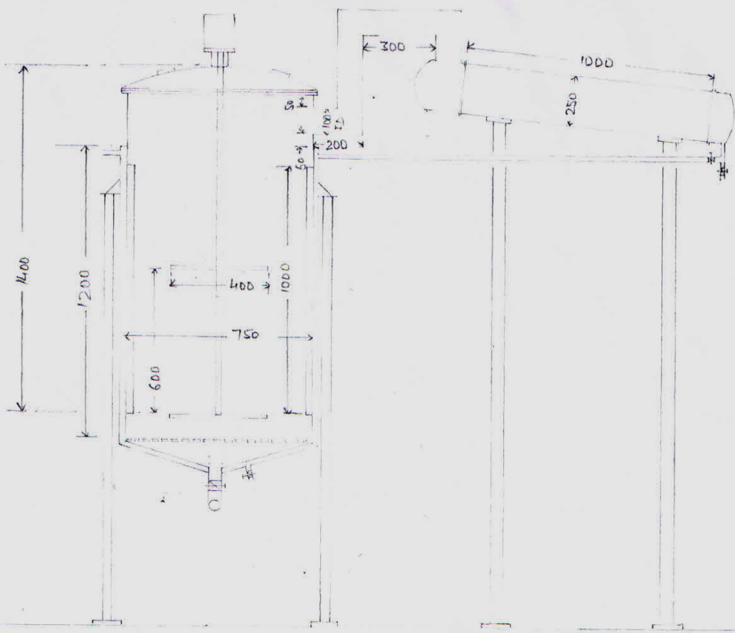
Extraction vessel, Capacity = 50 Litre / batch
